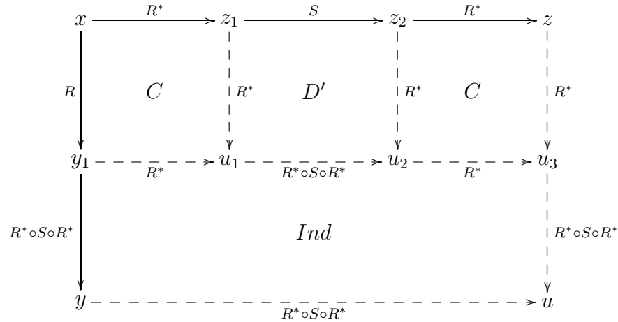
Figura 4.6.3: Caso xR \circ R^* \circ S \circ R^*y
