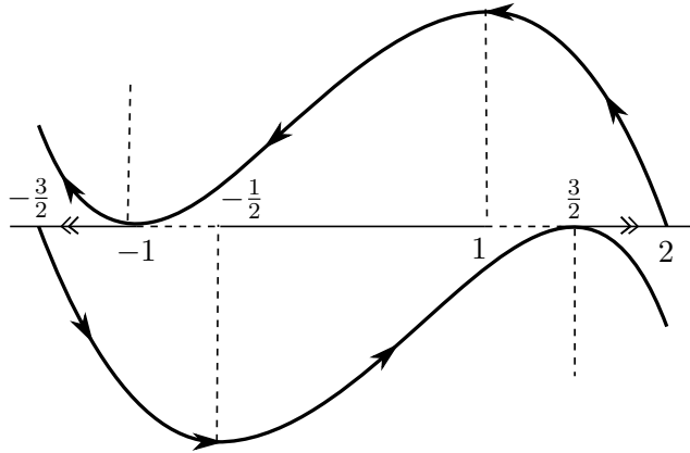
FIGURE 5. Periodic orbit (for positive time)
