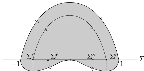
FIGURE 2. Chaotic set \Lambda .
