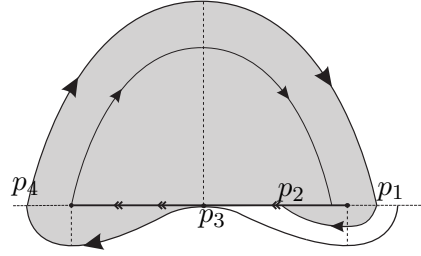
FIGURE 4. Positive chaotic set \tilde{\Lambda} .
