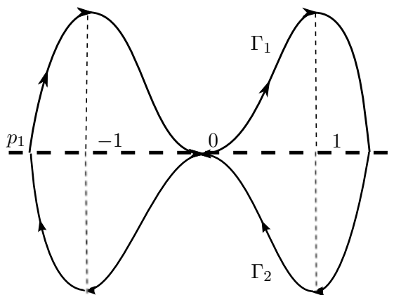
FIGURE 6. Trivial minimal set which is chaotic for Z
